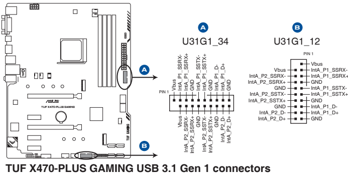
TUF X470-PLUS GAMING USB 3.1 Gen 1 connectors
