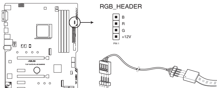
TUF X470-PLUS GAMING RGB Header
